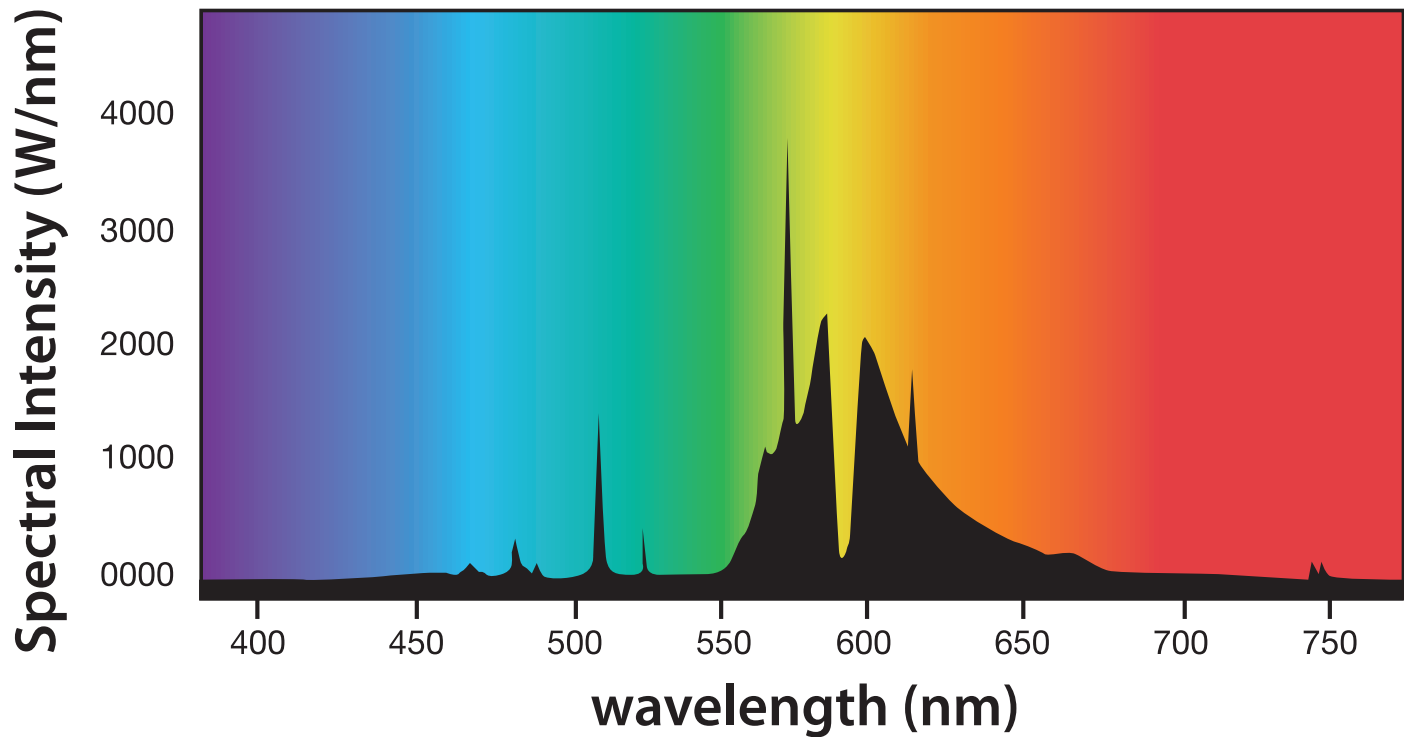
DigiMax 1000 Watt Double-Ended HPS Lamp - Spectral Intensity Graph
