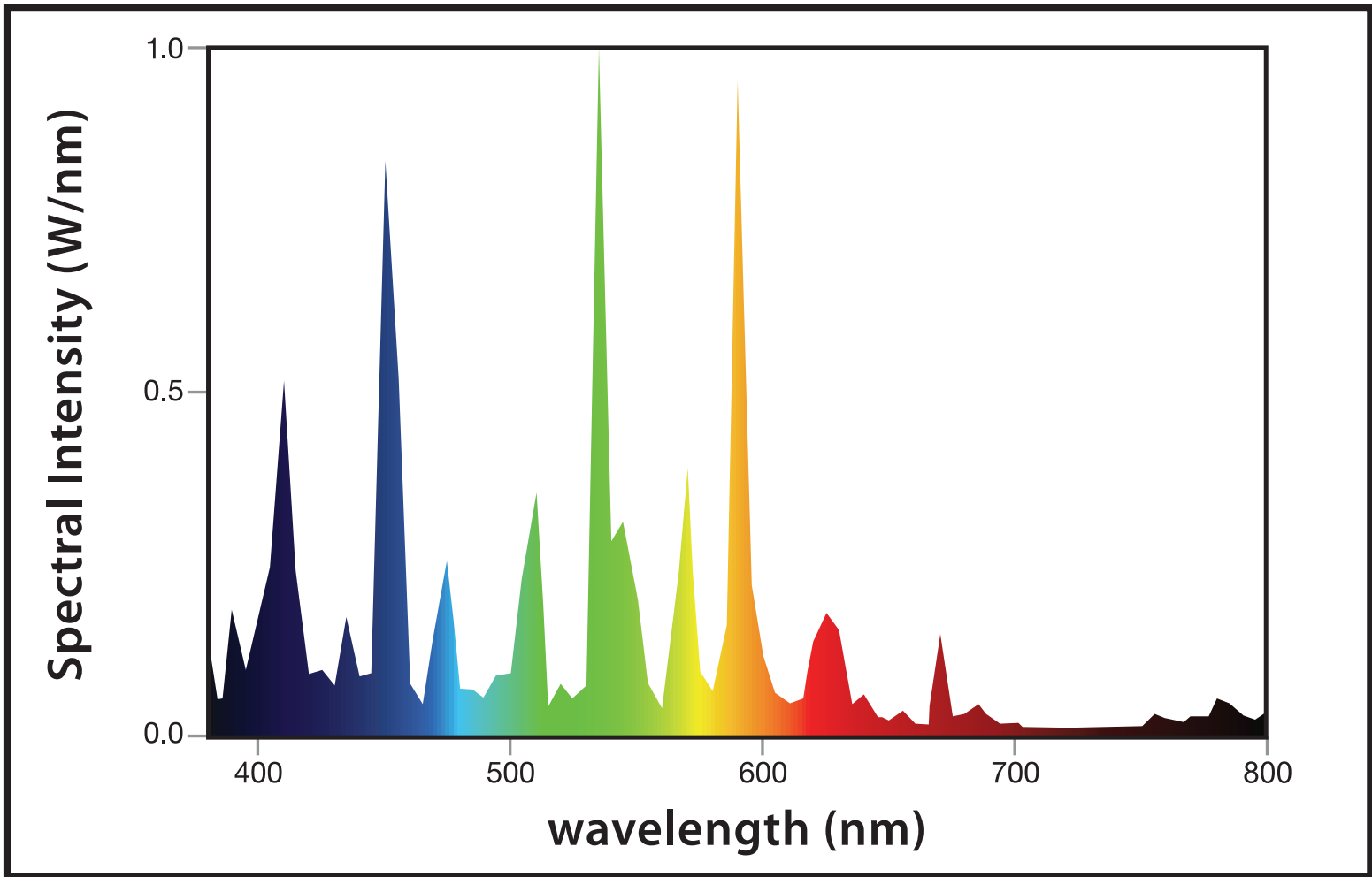
Ultra Sun 400 Watt - 7,500°K MH Lamp - Spectral Intensity Graph
