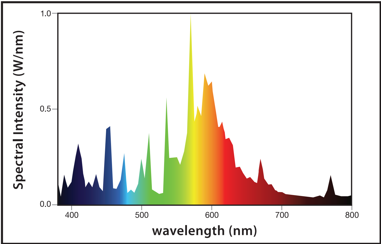
Ultra Sun 1000 Watt - Dual Arc Tube Lamp - Spectral Intensity Graph
