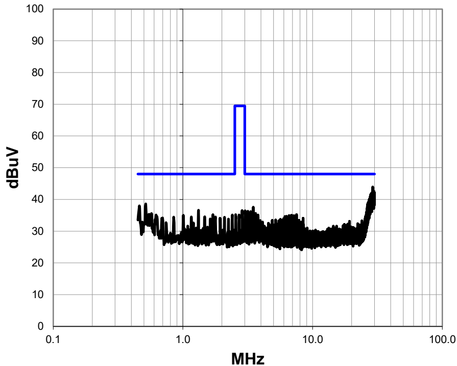
Peak Data - vs - Quasi Peak Limit
